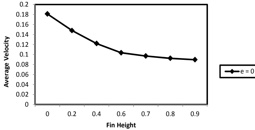
Fig. 10 Variation of average velocity with fin height . For e=0, H=0.2, F=4, \alpha=3^\circ, W=0.2
