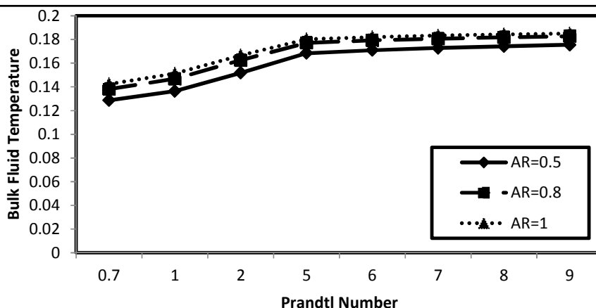
Fig. 14. Variation of Bulk fluid temperature with Prandtl number for different aspect ratios. For H=0.2, F=4, \alpha=3^\circ, W=0.2
