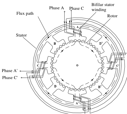
Figure 2. The cross-sectional views of the 1.8° hybrid stepping motor showing the PM flux and phase winding connections
