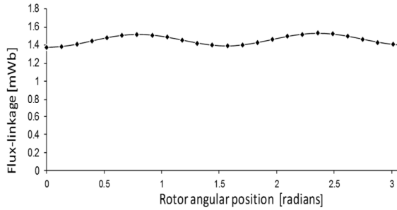
Figure 3: The permanent magnet flux-linkage measured from phase winding
