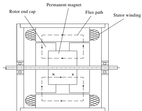
Figure 2. The cross-sectional views of the 1.8° hybrid stepping motor showing the PM flux and phase winding connections
