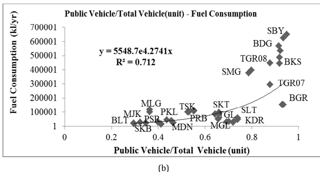
Figure 5. Relationship between public passenger vehicles - total fuel consumption (kl/year), Source: [2]
