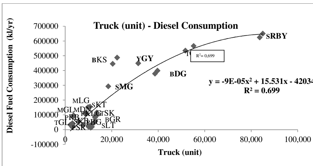
Figure 7. Relationship between truck – diesel fuel consumption, Source:[2]
