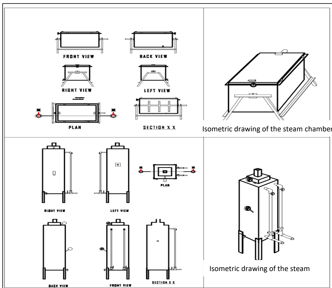
Fig.2. Orthographic projections of the steam parboiler
