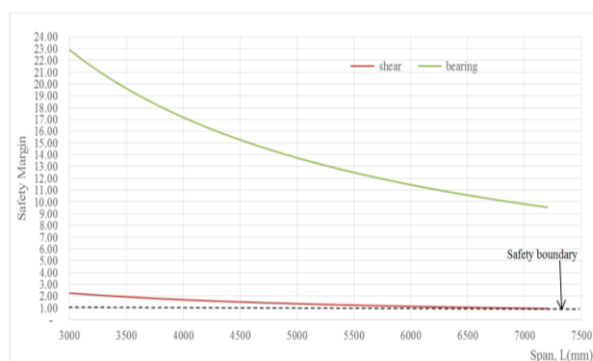
Figure 2 Variation in Span with the Safety Margin of Anogeissus Schimperi Timber Bridge Beam
