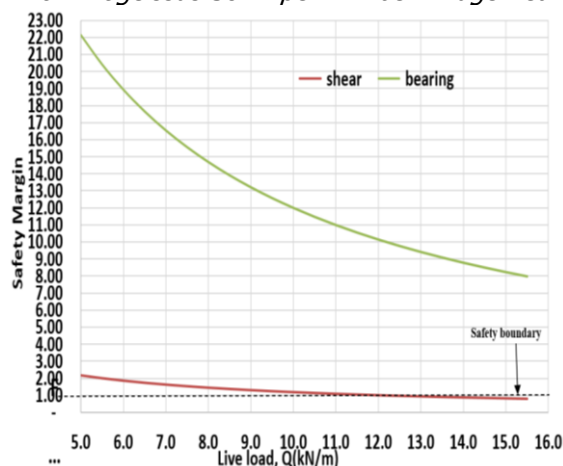
Figure 5: Variation in Live Load with the Safety Margin of Anogeissus Schimperi Timber Bridge Beam
