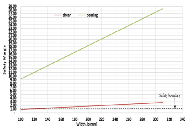
Figure 4: Variation in Width with the Safety Margin of Anogeissus Schimperi Timber Bridge Beam
