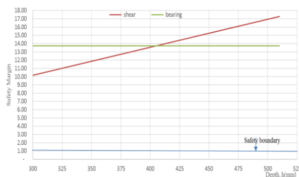
Figure 3 Variation in depth with the Safety Margin of Anogeissus Schimperi Timber Bridge Beam
