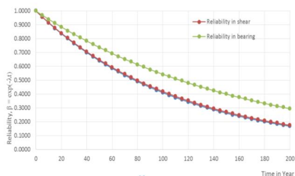
Figure 1: Reliability of Anogeissus schimperi Timber Bridge Beam
